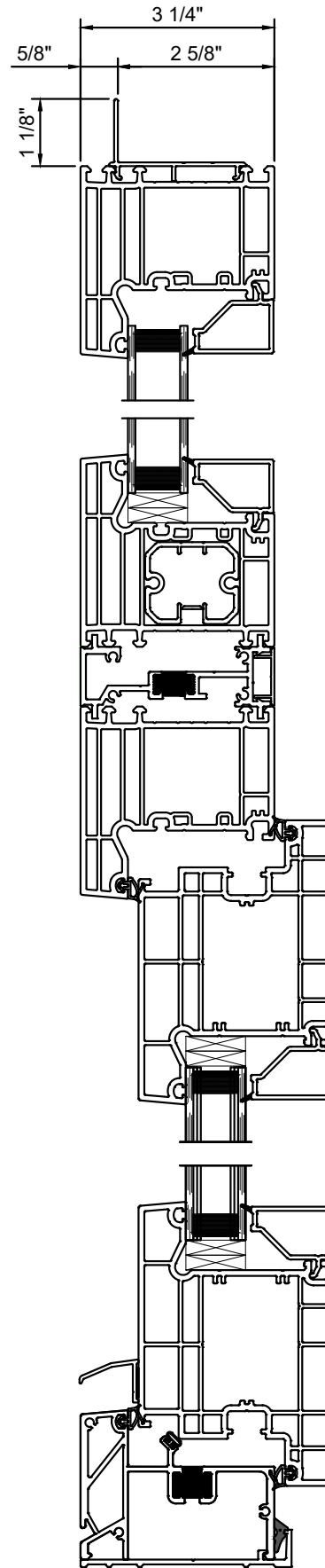
In-Swing Door w/ Transom
