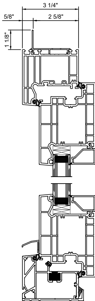
In-Swing Door w/o Transom
